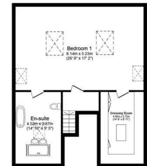
Second Floor Floor area 72.7 sq.m. (783 sq.ft.)
